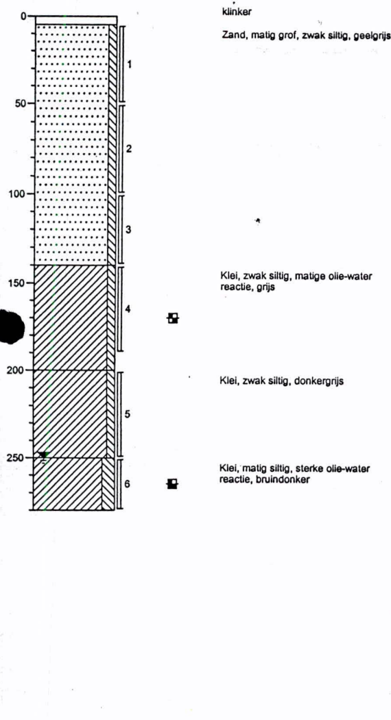
Boring: 108
