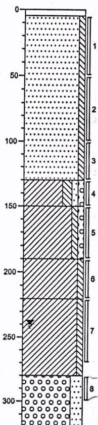
Boring: 101
