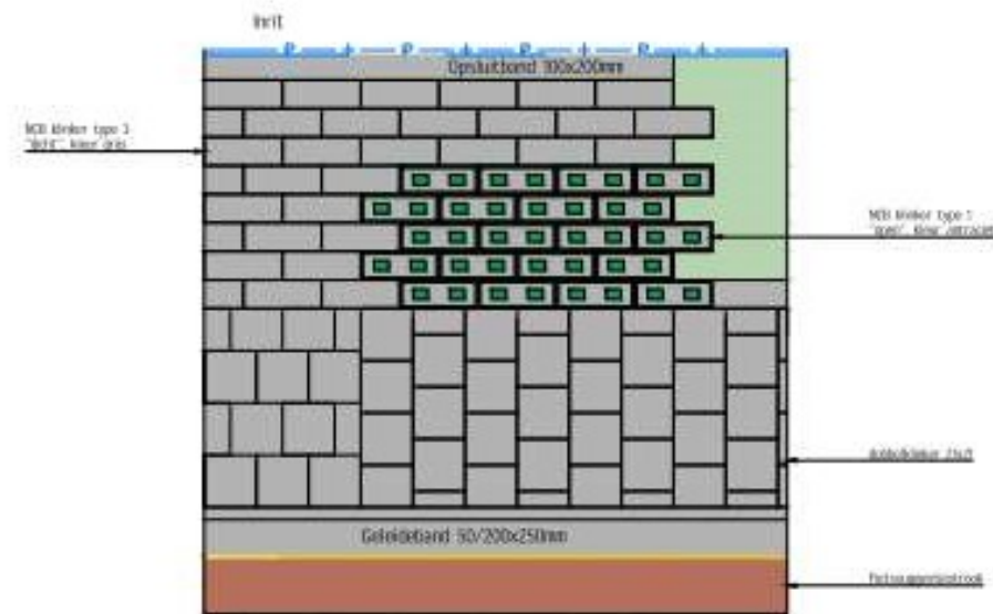
Principe detail 02: NCB klinkers Schaal 1:20
