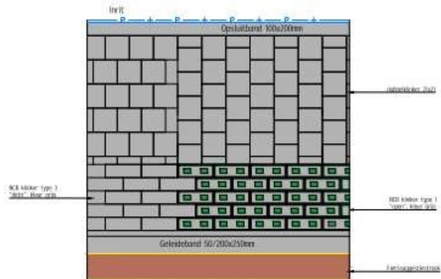
Principe detail 01: NCB klinkers Schaal 1:20
