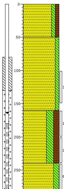
Boring: 103
