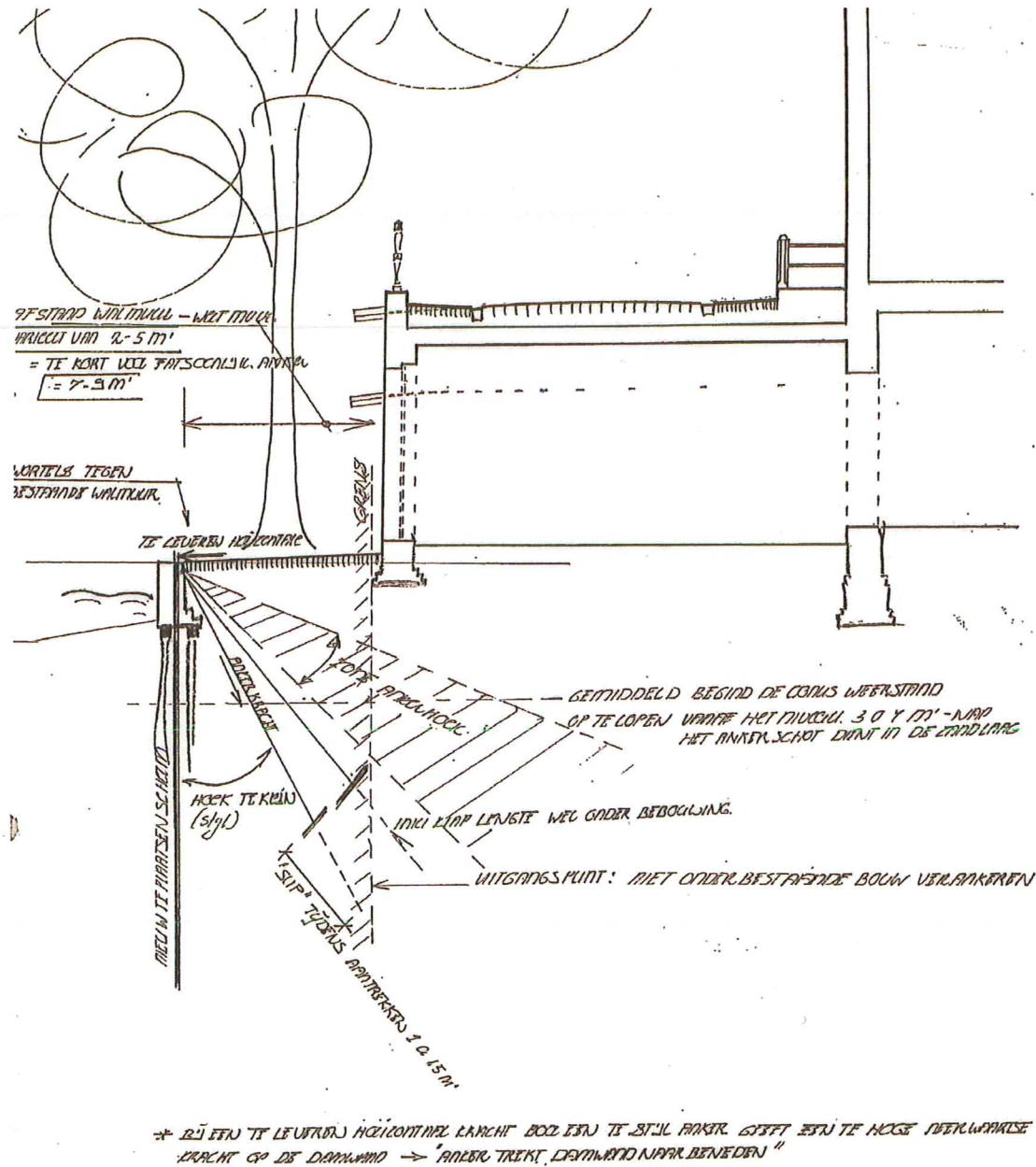
Schets verankerde houten damwand
