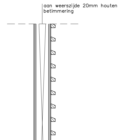
Detail V 1:20
