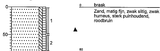
Boring: 03
